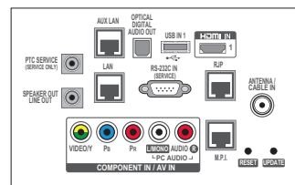
REAR JACK PANEL
