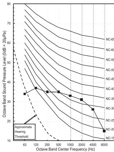
ARNU12GVEA4
