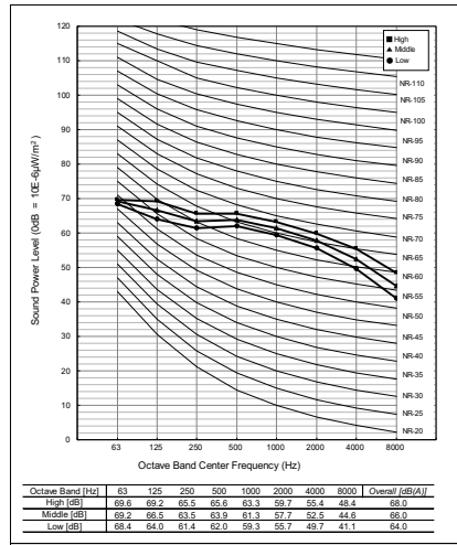
ARNU54GM3A4
