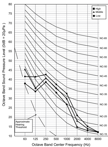
ARNU24GTBB4
