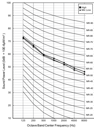
ARNU76GB8A4
