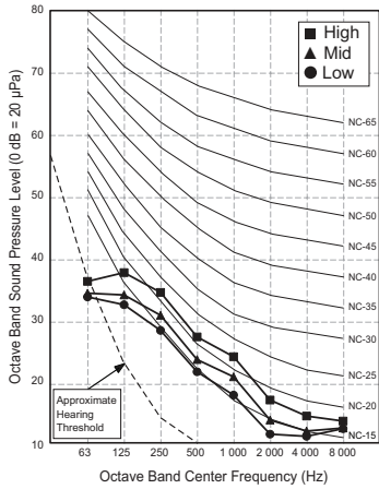
ARNU21GL3G4
