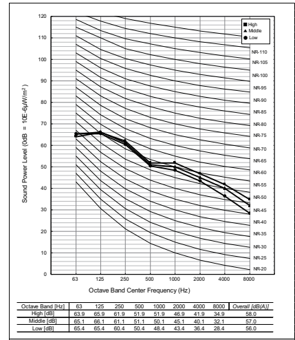
ARNU24GM1A4
