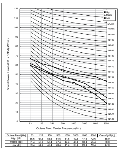
ARNU15GM1A4
