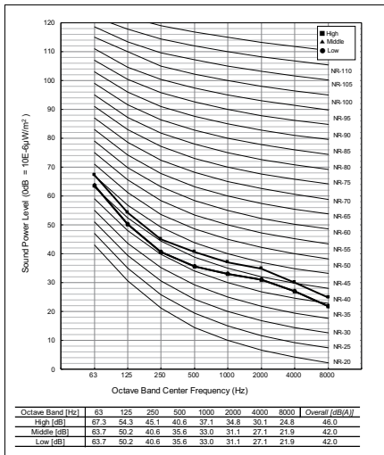
ARNU76GB8Z4
