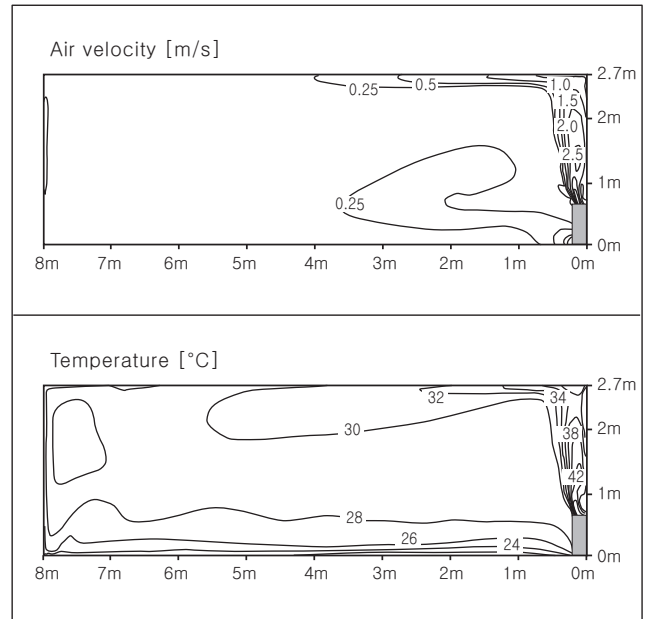
Heating
