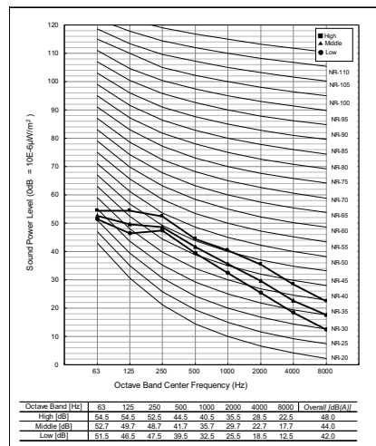
ARNU09GM1A4
