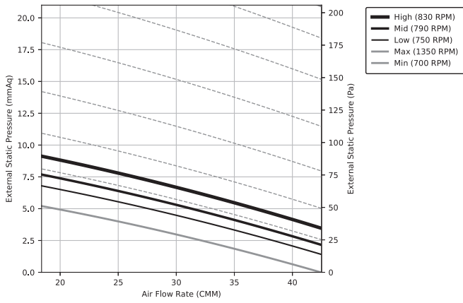
PQ Curve
