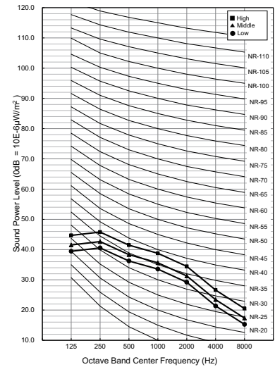
ARNU07GL4G4
