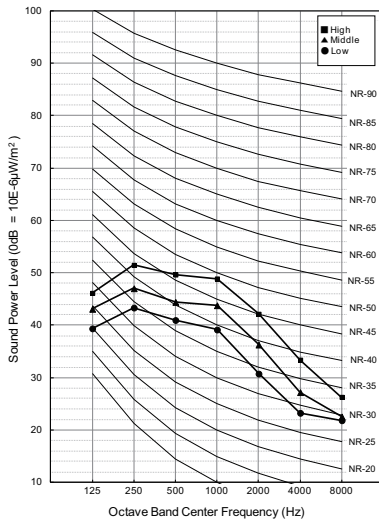
ARNU07GCEA4 ARNU07GCEU4
