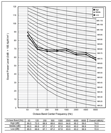
ARNU96GB8Z4
