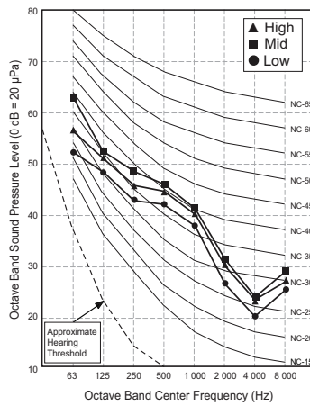
ARNU42GB8A4
