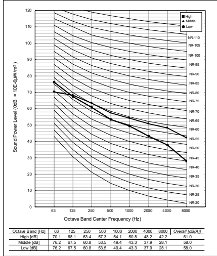
ARNU96GB8Z4
