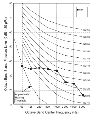
ARNU12GCEA4 ARNU12GCEU4
