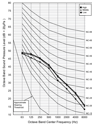
ARNU54GM3A4
