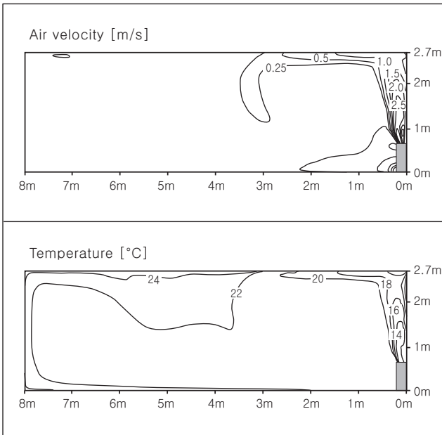
Cooling
