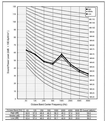
ARNU42GM2A4
