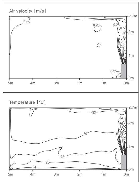
Heating
