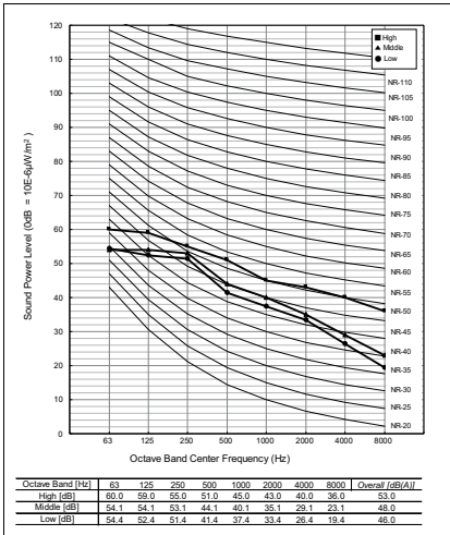
ARNU15GM1A4
