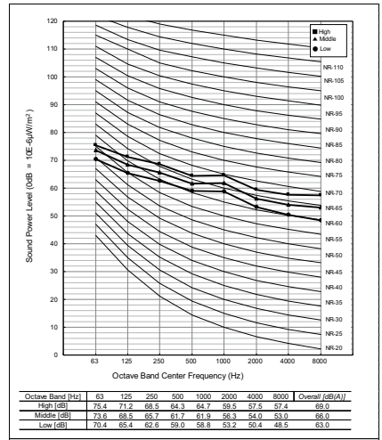
ARNU42GM2A4
