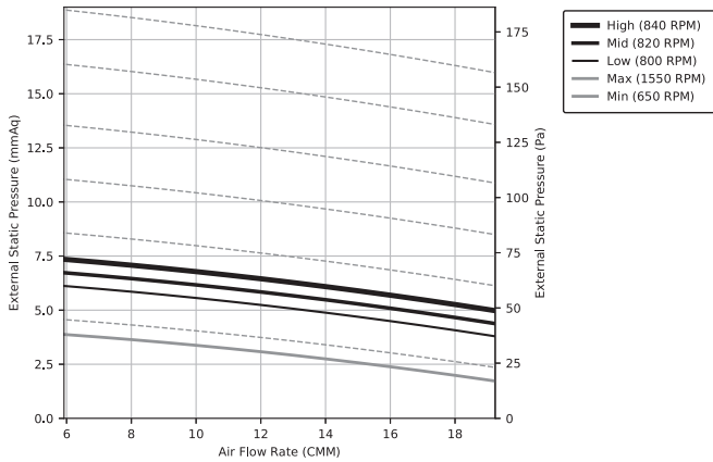
PQ Curve
