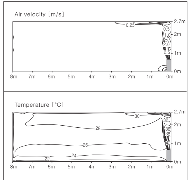
Heating
