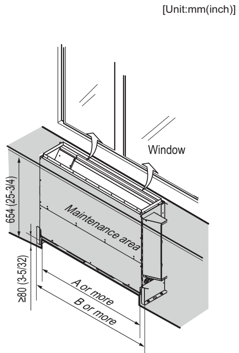
Without Case
