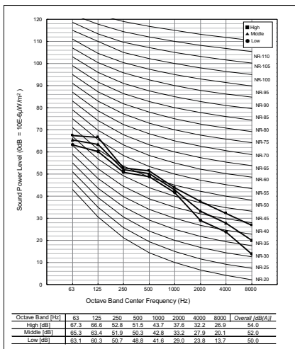
ARNU48GM3A4
