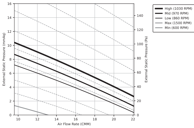
PQ Curve
