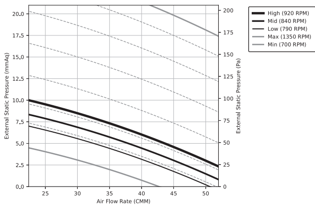
PQ Curve
