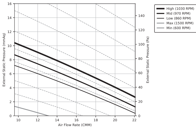
PQ Curve
