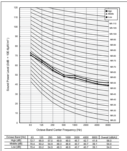
ARNU76GB8Z4
