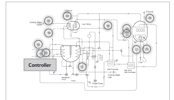
Piping Diagram
